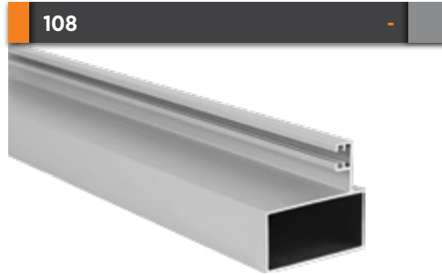
Oluklu Büyük Kasa Profil Corrugated Big Case Profile Paket İçi Adet Amount within package 3 Gramajı Weight 1,611 kg/m
