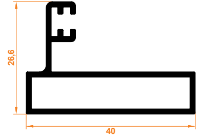
Dar Yan Dikme Thin Side Column
