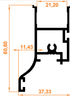
Sabit Panel Yan Dikme Profil Fixed Panel Side Column Profile
