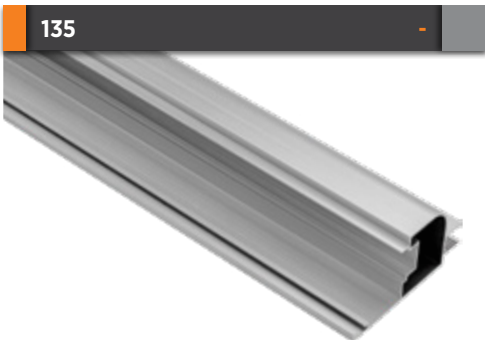
8 mm İspanyolet Profil 8 mm Espagnolette Profile Paket İçi Adet Amount within package 6 Gramajı Weight 0,517 kg/m
