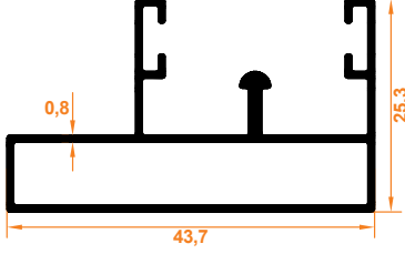
Aykim Kasa Profil Aykim Case Profile
