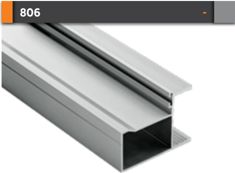
806 90° Dönüş Profil 90° Return Profile Paket İçi Adet Amount within package 6 Gramajı Weight 0,475 kg/m
