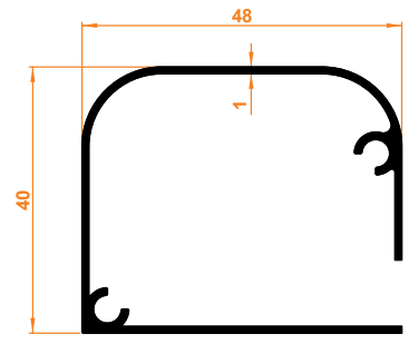
Store Kasa Profil Store Case Profile
