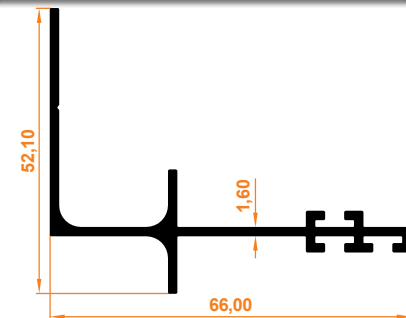
Yan Ray "L" Profil Side Rail "L" Profile
