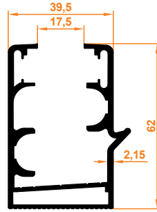
Oluklu Kasa Profil Corrugated Case Profile
