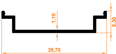
Ray Kapatma "L" Profil Rail Closure "L" Profile
