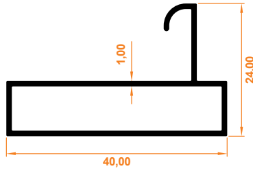
Store Alt Kasa Profil Store Bottom Case Profile
