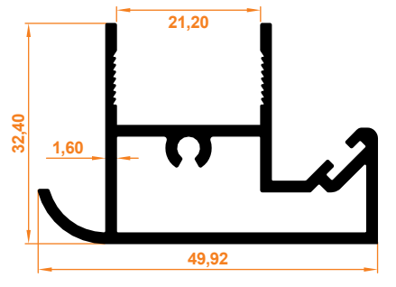
Sabit Panel Üst Baza Profil Fixed Panel Top Base Profile
