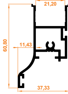
Sabit Panel Yan Dikme Profil Fixed Panel Side Column Profile
