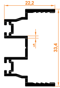
Düz Kapak Menteşe Profil Flat Cover with Hinge Profile
