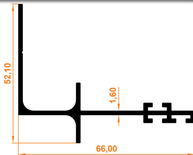
Yan Ray "L" Profil Side Rail "L" Profile
