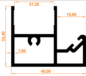
Kenet Kasa Profil Clamp Base Profile
