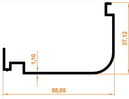
Ray Kapatma "T" Profil Rail Closure "T" Profile
