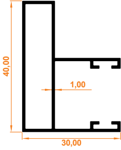
Store Yan Kasa Profil Store Side Case Profile
