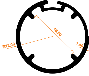
Store Boru Profil Store Pipe Profile
