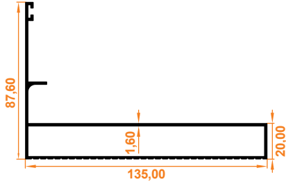
Yan Kasa Profil Side Case Profile
