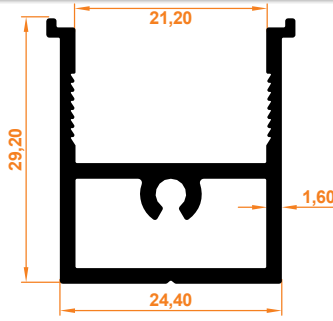
Hareketli Panel Yan Dikme Profil Movable Panel Side Column Profile
