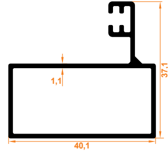
Geniş Yan Dikme Thick Side Column Profile
