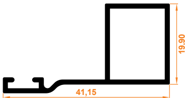
Kasa Profil Case Profile
